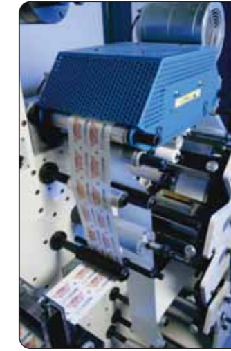
TENSION CONTROL
