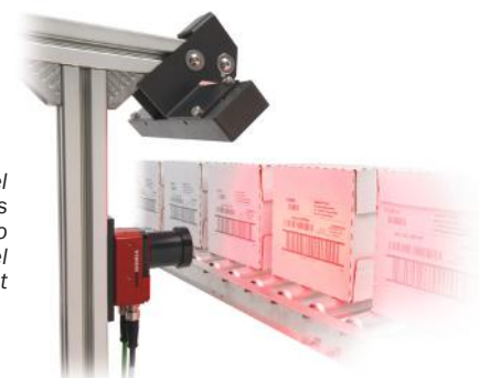
Figure 12: A label verification system is installed on the line to ensure consistent label codes and print quality at production speeds.
